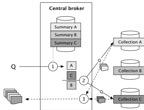
Fig. 1. Schematic overview of a typical broker-based distributed information retrieval system
