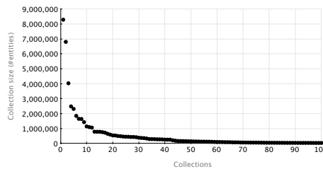
Fig. 3. Distribution of collection sizes in BTC-2009
